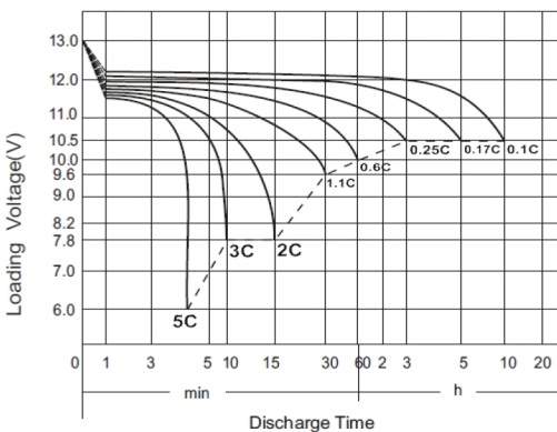
Discharge Characteristics
