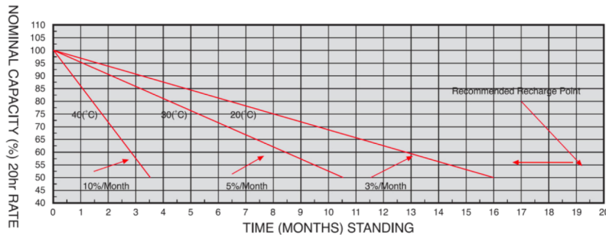
Discharge Characteristics
